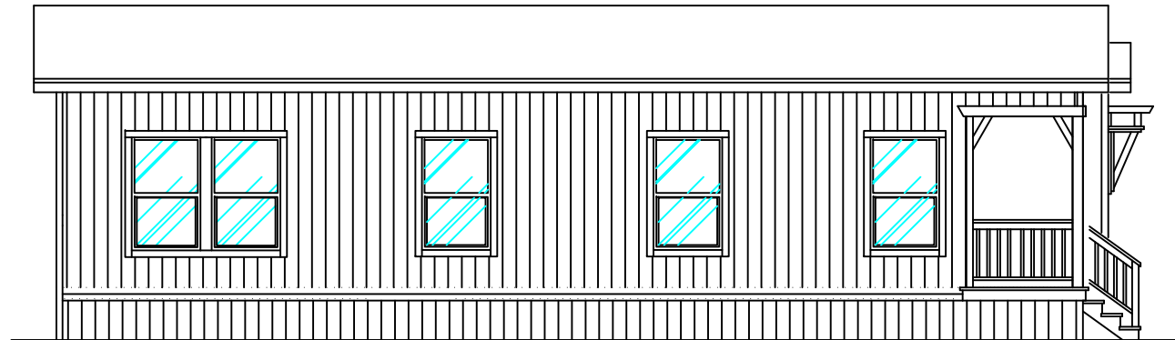
SIDEWALL ELEVATION - LEFT
