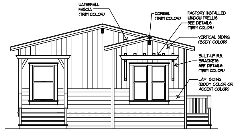
ENDWALL ELEVATION - FRONT (ALT. ENTRY)
