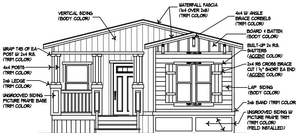
ENDWALL ELEVATION - FRONT (STD)
