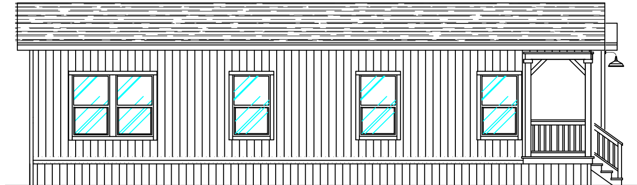
Left Side Elevation ( FARMHOUSE)
