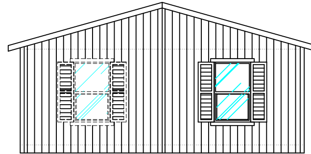
FRONT ENDWALL ELEVATION - STD (SHOWN WITH OPT. B3 WINDOW)
