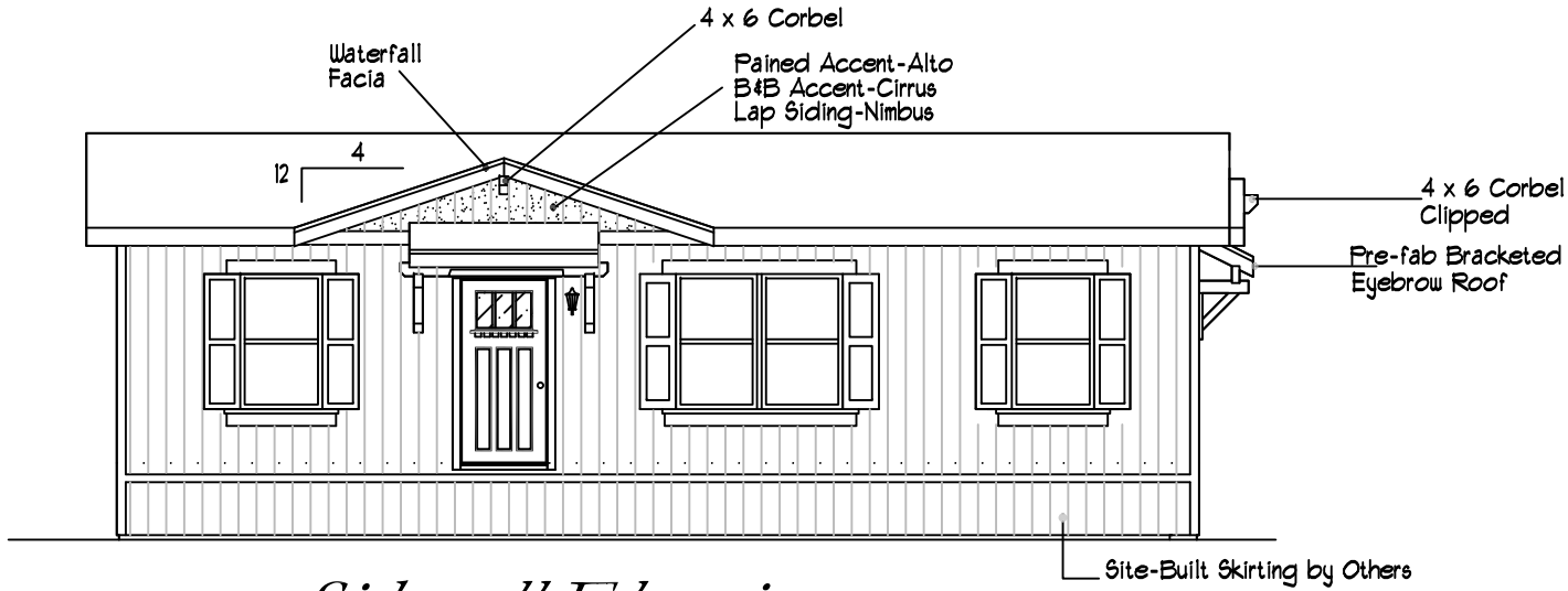
Sidewall Elevation
